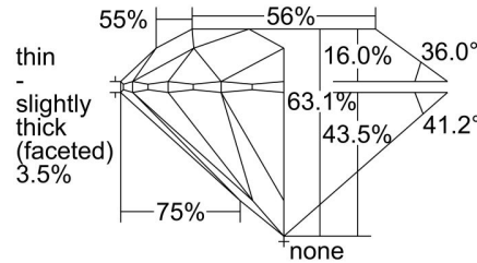
Cut grade affected by brillianteering
